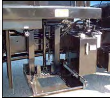
Optional vibratory plate hydraulic platform to reduce back injuries relating to lifting hazards.
